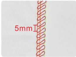
大针距设计提升送料效率 Large needle guage design, improve feeding efficiency
