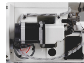
步进电机驱动抬压脚和剪线 Step motor drive foot lifter and trimming
