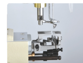
智慧型差动微调器可精密调整差动量 Micro-adjustment regulator makes differential feed ratio easy and precise.
