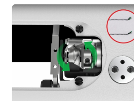
双刀剪线，短线头迹迹美观 Dual-cutter trimming produces short thread ends and neat stitches
