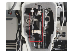
智能中压脚结构 Intelligent middle presser foot structure
