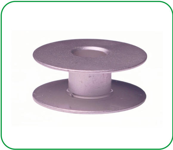
名称: 梭芯 Description: Bobbin 代码/Part No: 10025484 适配: A6000/A8100/A8130/A5310/A8200L Machine Type: A6000/A8100/A8130/A5310/A8200L
